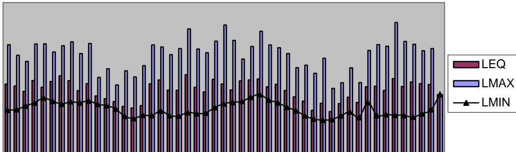
Figure 5. Noise Monitoring Data SLM-4 24559 Johnson St.
