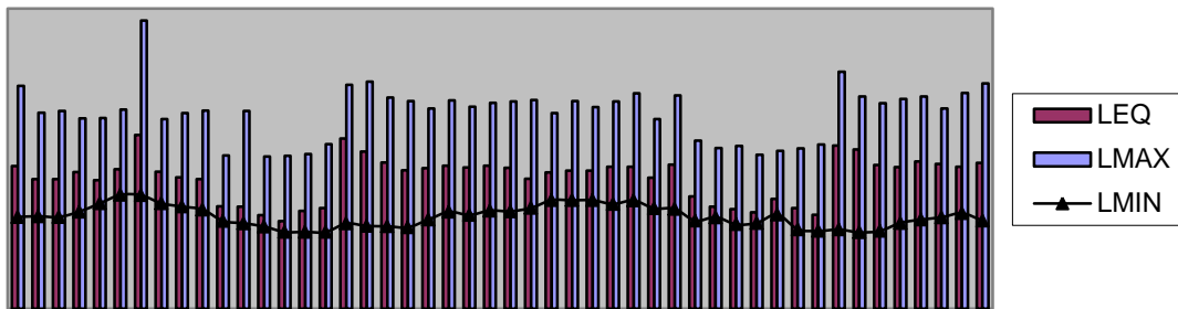
Figure 2. Noise Monitoring Data SLM-1 62 Soaring Eagle Road
